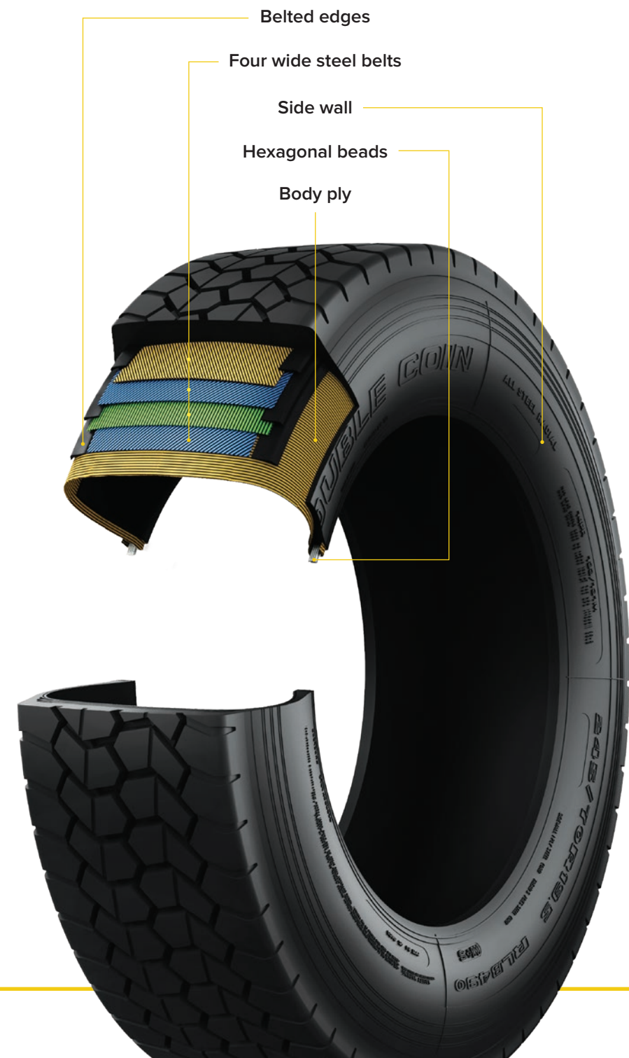
Diagram of tire construction
